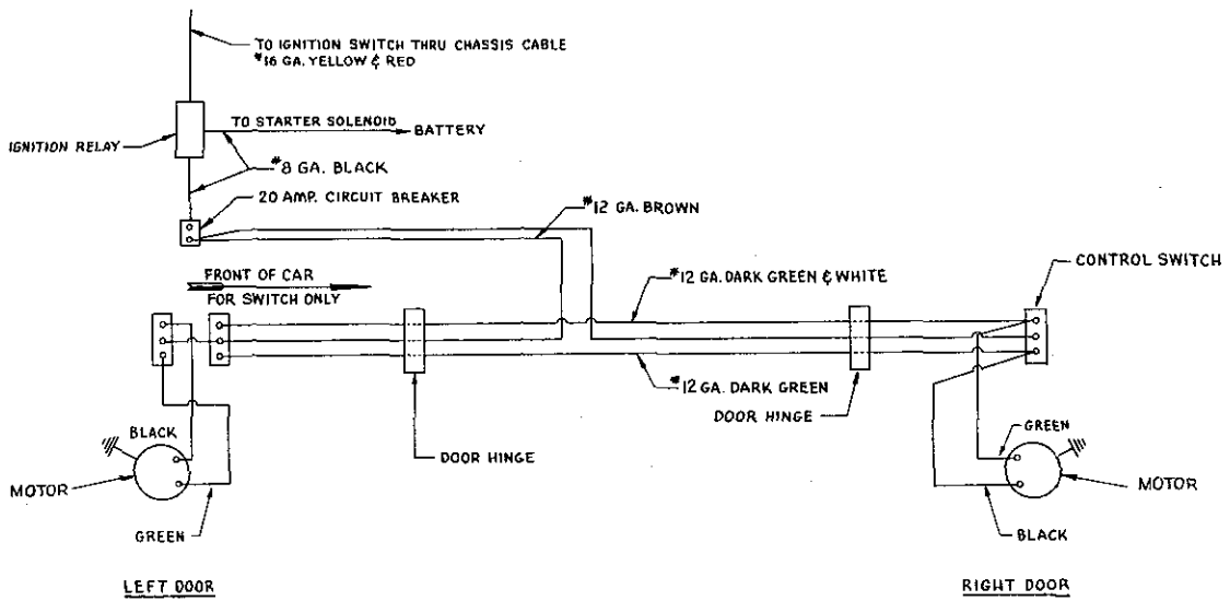
Wiring diagram—All models except 4 door sedans
